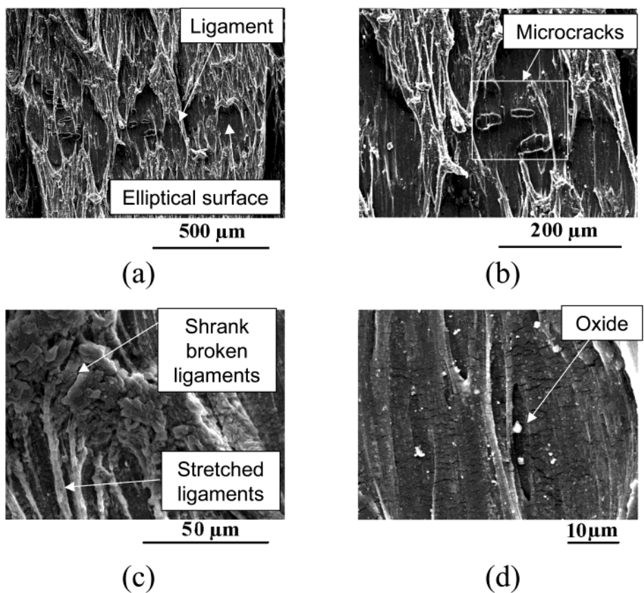
Figure 5. Details of the crack tip for four magnifications.
